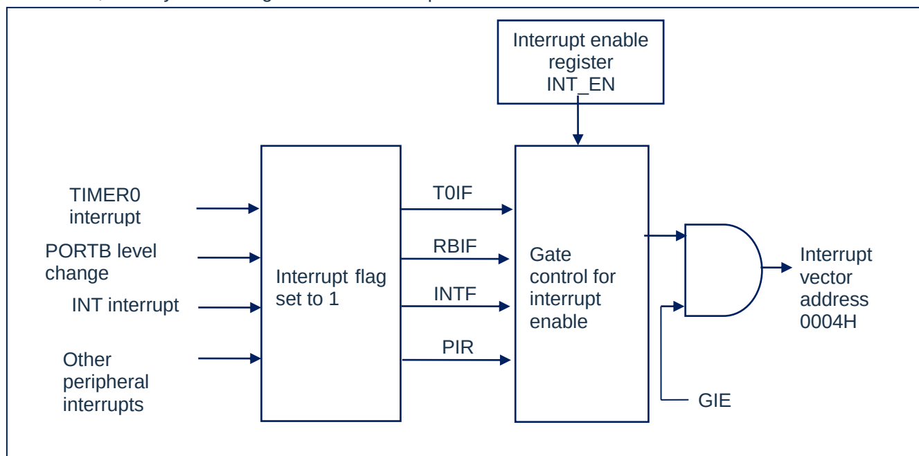
Figure 7-1: Schematic diagram of interrupt principle
